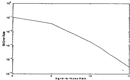
Fig.2 BER performance for the AM method
