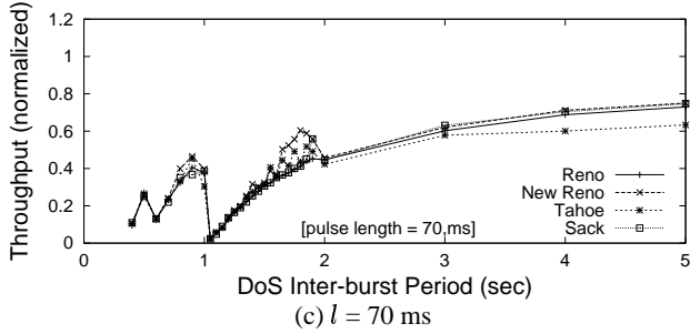
Figure 12: TCP Reno, New Reno, Tahoe and SACK under shrew DoS attacks
