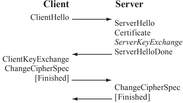
Figure 3: TLS Handshake —The client and server exchange messages to establish a shared master_secret, from which they derive cipher and MAC keys. The handshake ends with each side sending a Finished message, encrypted with the negotiated keys, that includes an integrity check on the entire handshake. The ServerKeyExchange message may be omitted, depending on the key exchange method in use.
