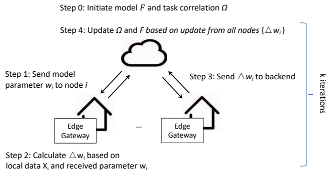
Fig. 8: Federated Multi-Task learning workflow.
