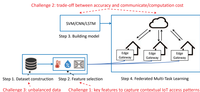
Fig. 9: Basic building blocks for LoFTI.
