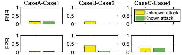
Fig. 19: FNR/FPR on unknown/known IoT attacks.
