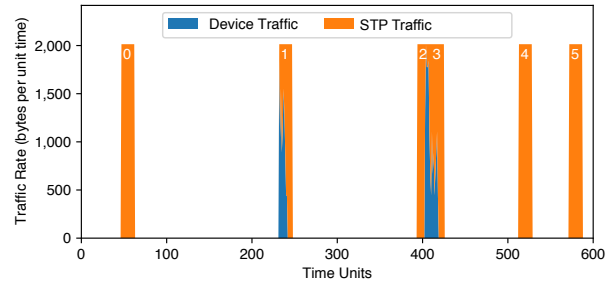
Fig. 3. Example of STP applied to smart outlet traffic. An adversary could not distinguish which periods of padding mask real device traffic corresponding to user activities.
