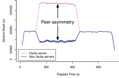
Figure 2: Peer-asymmetry of rd_sec for iozoner workload with disk-hog fault.
