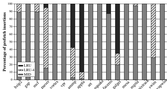
Figure 8. Distribution of the insertion position of prefetched blocks
