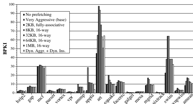
Figure 12. Bandwidth consumption of prefetch cache vs. FDP
