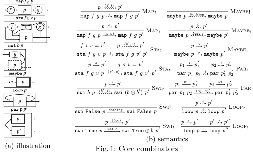
Fig. 1: Core combinators
