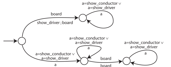
Fig. 1. An insertion automaton that effectively enforces the cable-car policy
