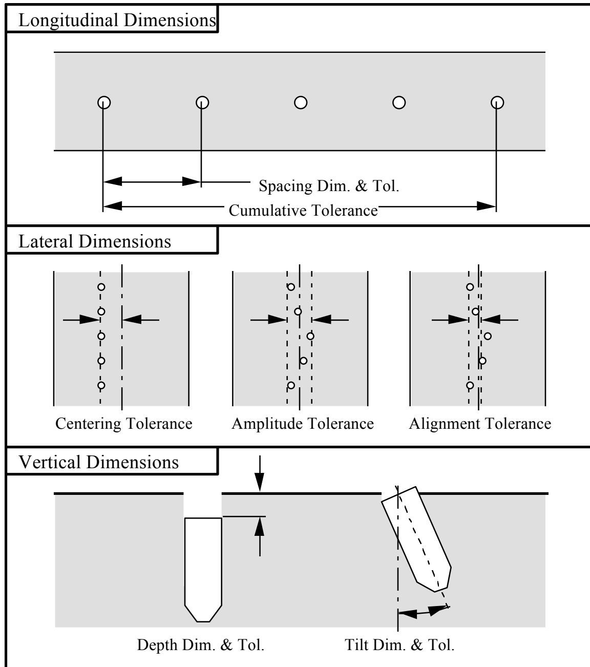
Figure 3. Illustration of dimensions & tolerances.
