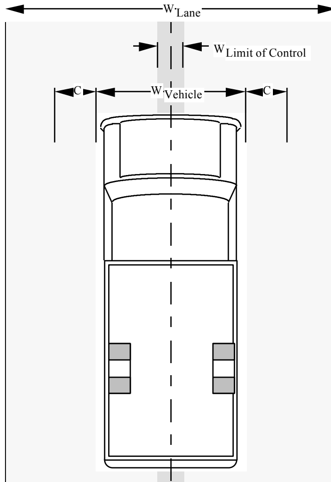
Figure 4. Limit of control width & other centering factors.
