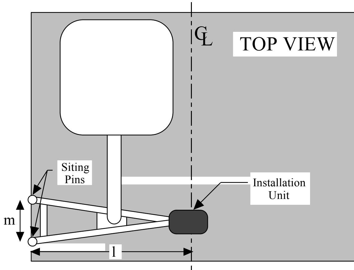
Figure 15. Ruled edge locator.
