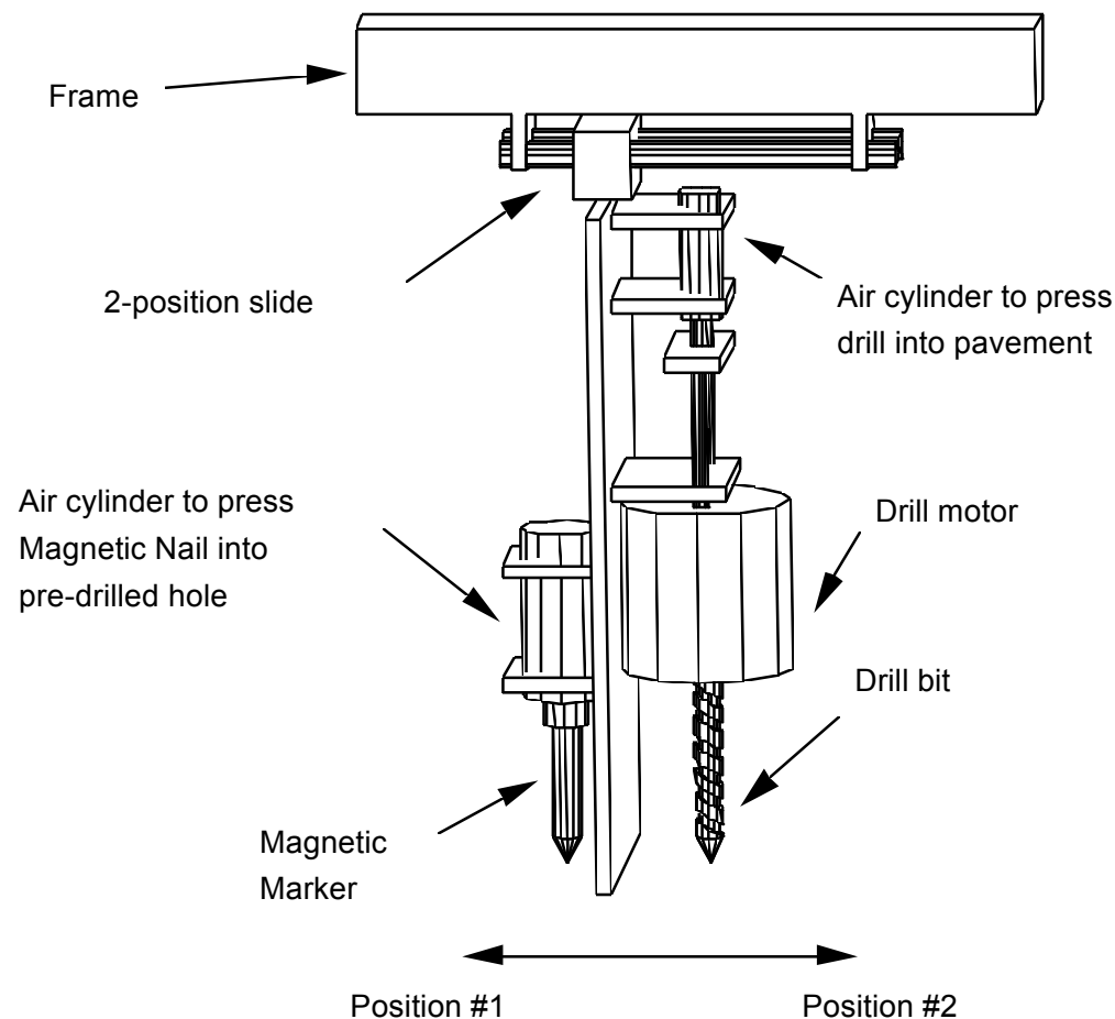
Figure 29. Drill-then-Press unit.
