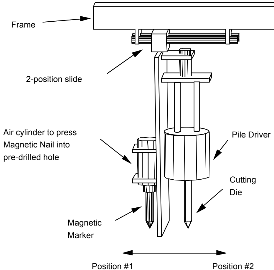
Figure 32. Translating pound-then-press unit.
