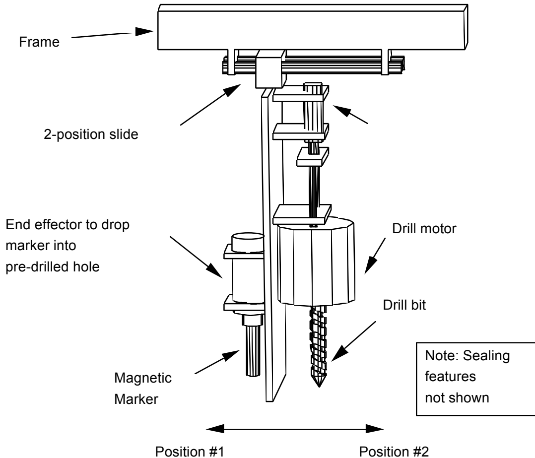
Figure 30. Drill-then-Place unit.
