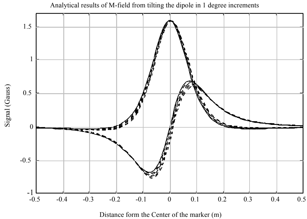
Figure 7. Sensed signal for dipole tilted in 1^\circ increments.
