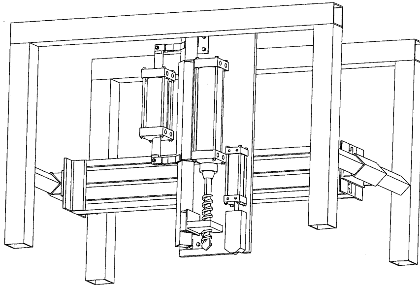
Figure 58. The magnetic nail placement mechanism.
