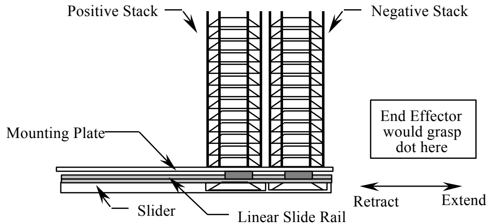
Figure 43. The gravity-loaded dot feeder.
