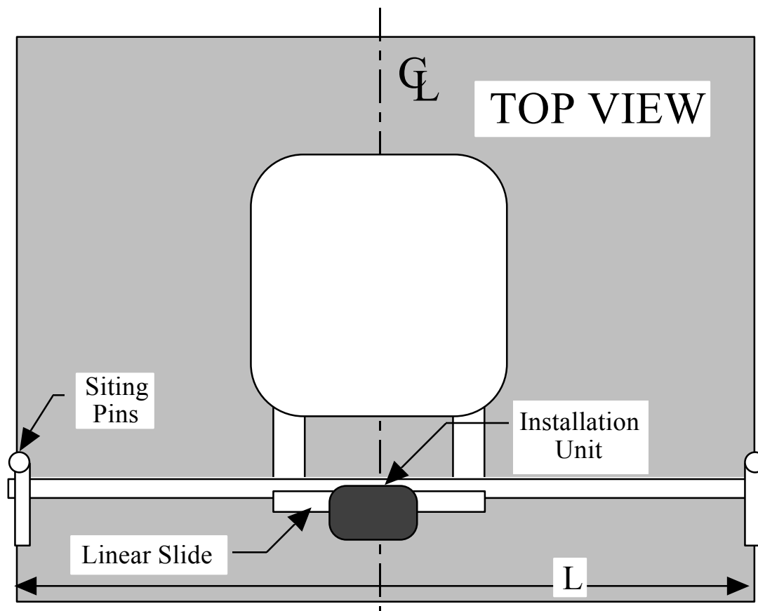
Figure 16. Averaged edge reference locator.
