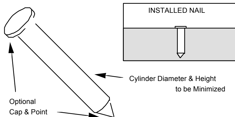
Figure 9. Magnetic nail marker.
