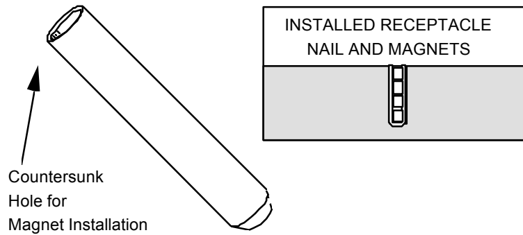
Figure 13. Receptacle nail.
