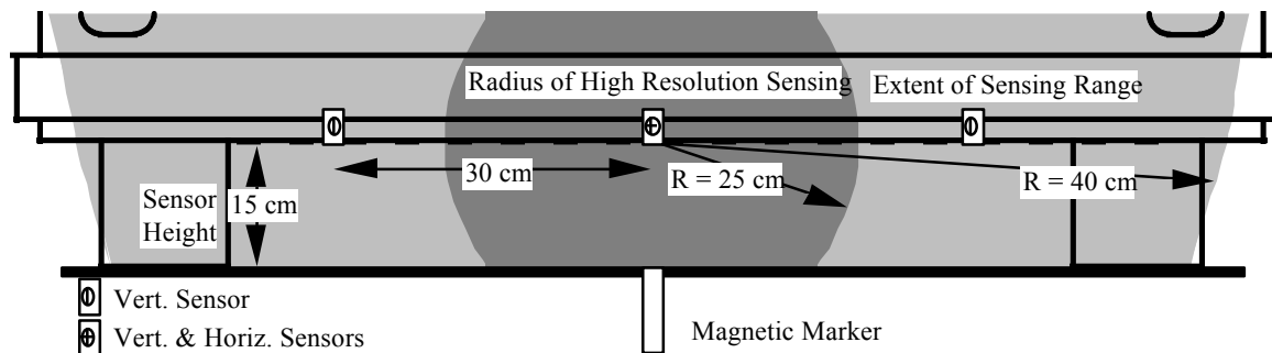
Figure 1. Range of sensors.
