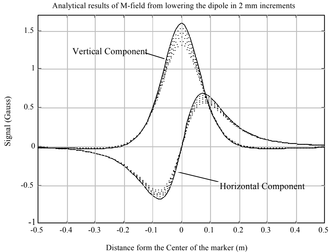
Figure 6. Sensed signal for dipole at different installation depths.
