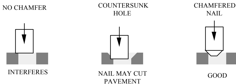
Figure 10. Effects of chamfering technique.
