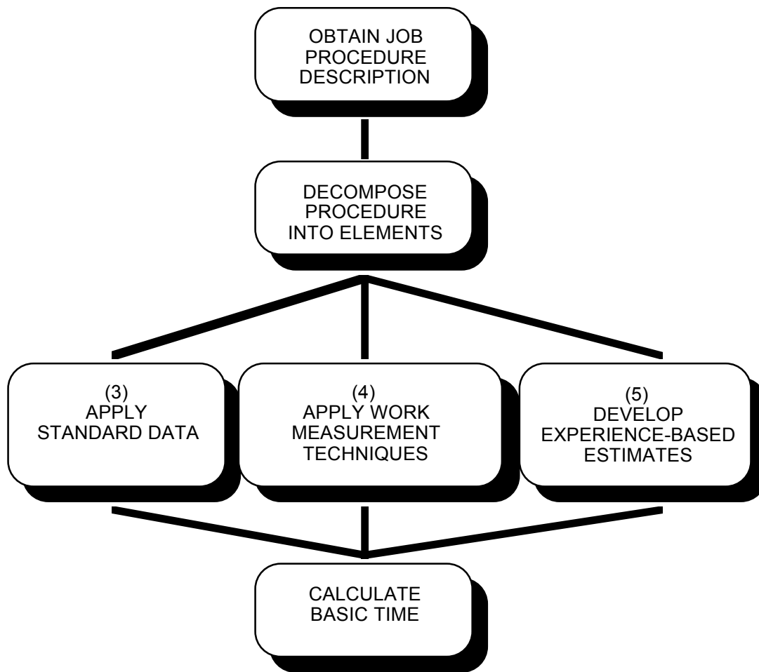
Figure 49. Analytical manpower estimation procedure.
