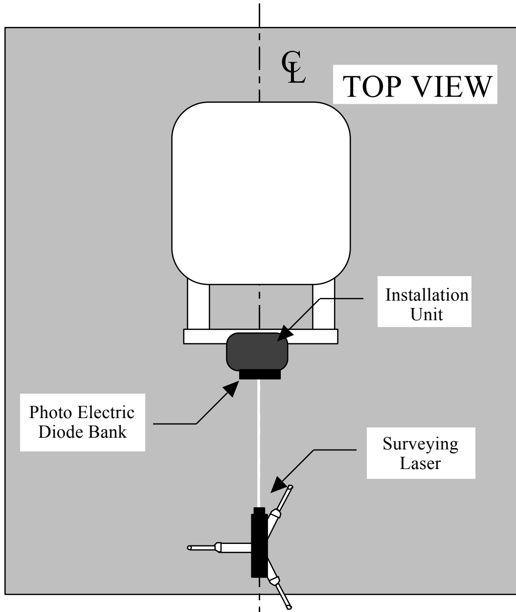
Figure 28. Laser-guided centering.
