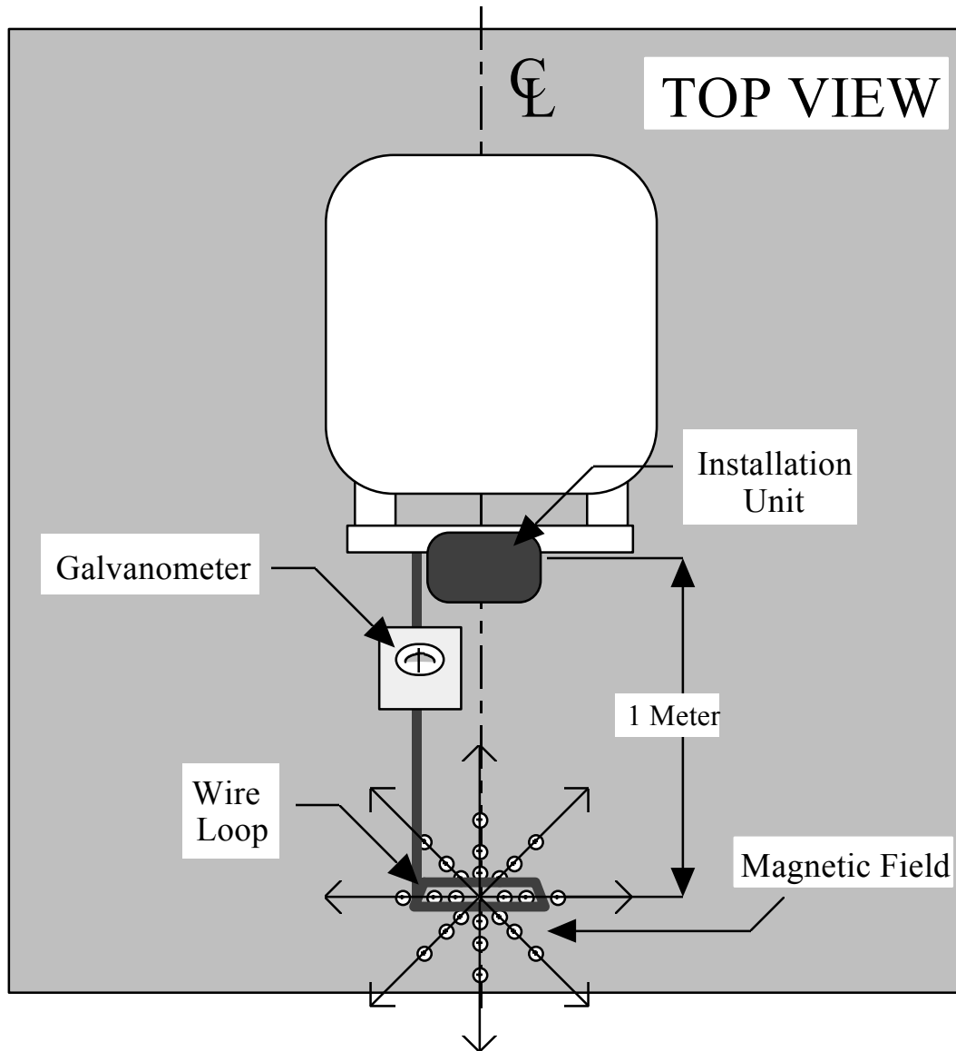
Figure 22. Galvanometer System.
