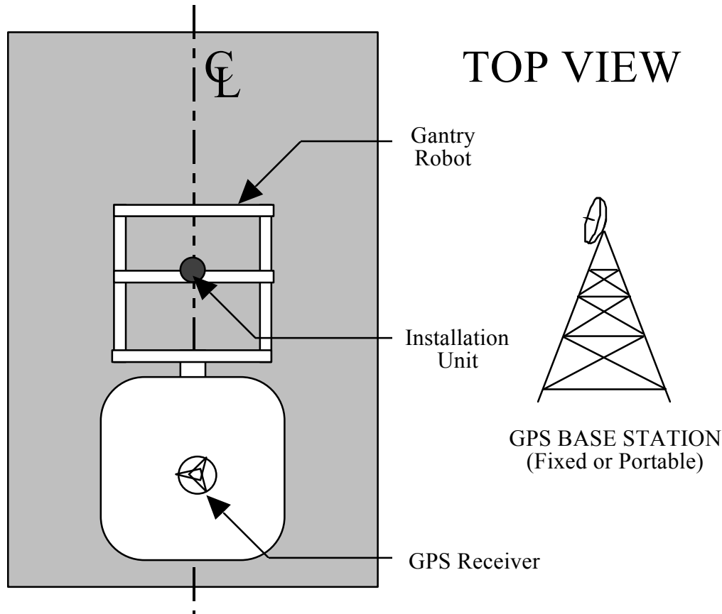
Figure 24. Installation using D-GPS.
