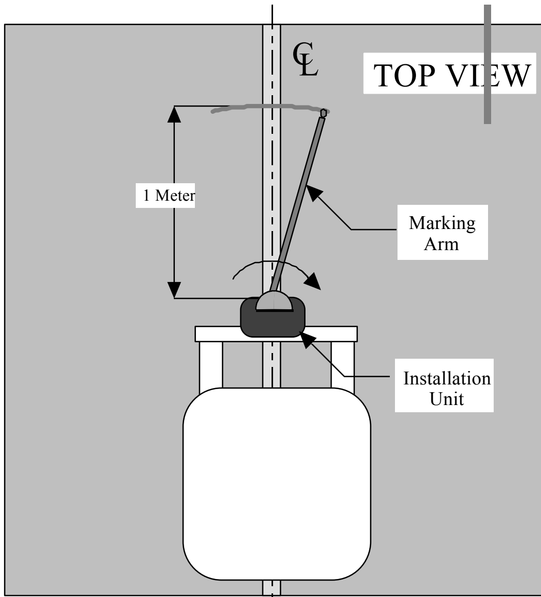
Figure 18. Forward “Compass” ruled measure.
