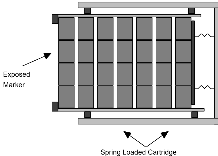
Figure 39. Loaded cartridge system powered with springs.
