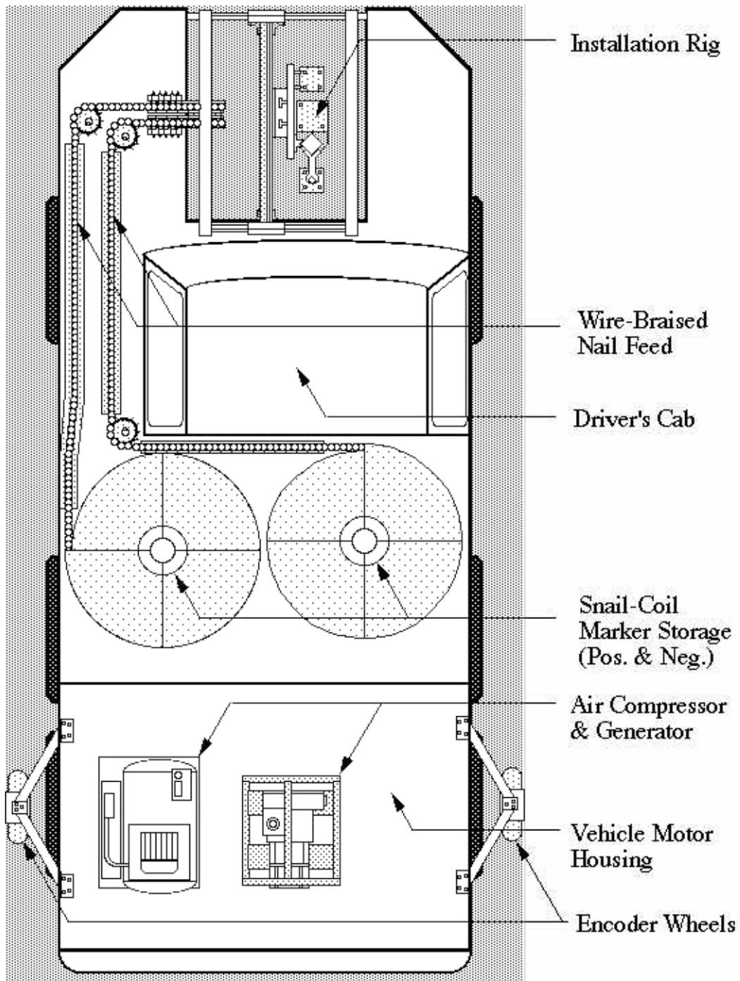
Figure 44. Prototype discrete magnetic marker placement truck.
