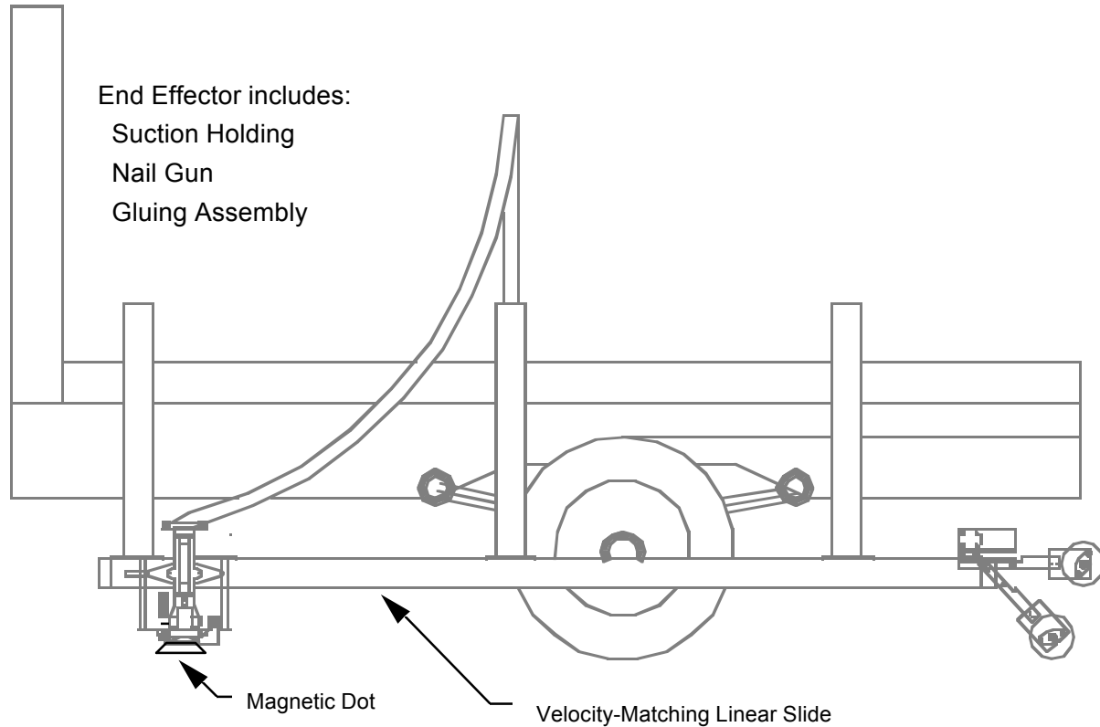
Figure 31. Continuous dot layer.
