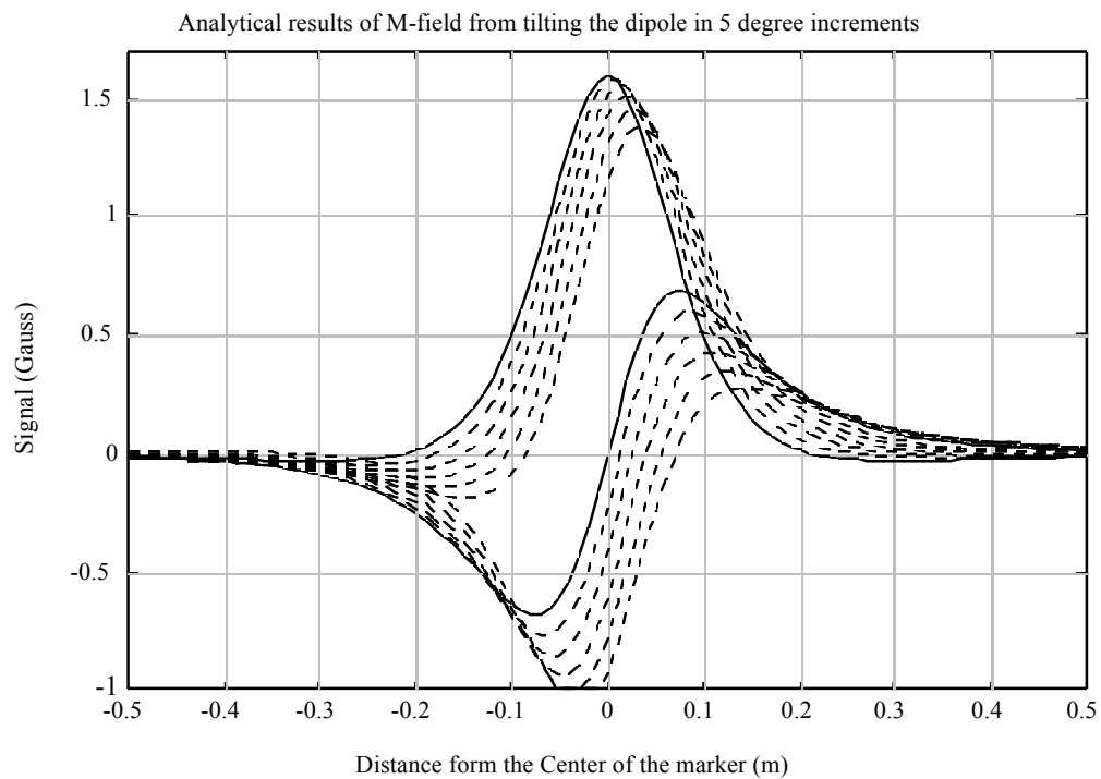
Figure 8. Sensed signal for dipole tilted in 5^\circ increments.
