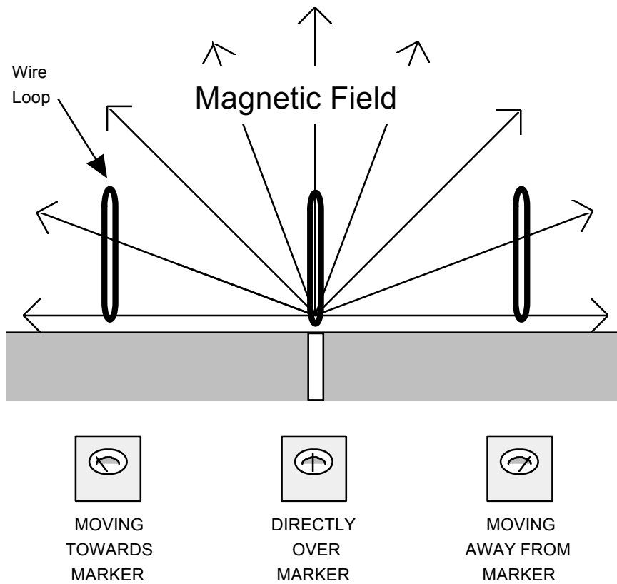
Figure 23. Galvanometer readings as wire loop moves through M-Field.
