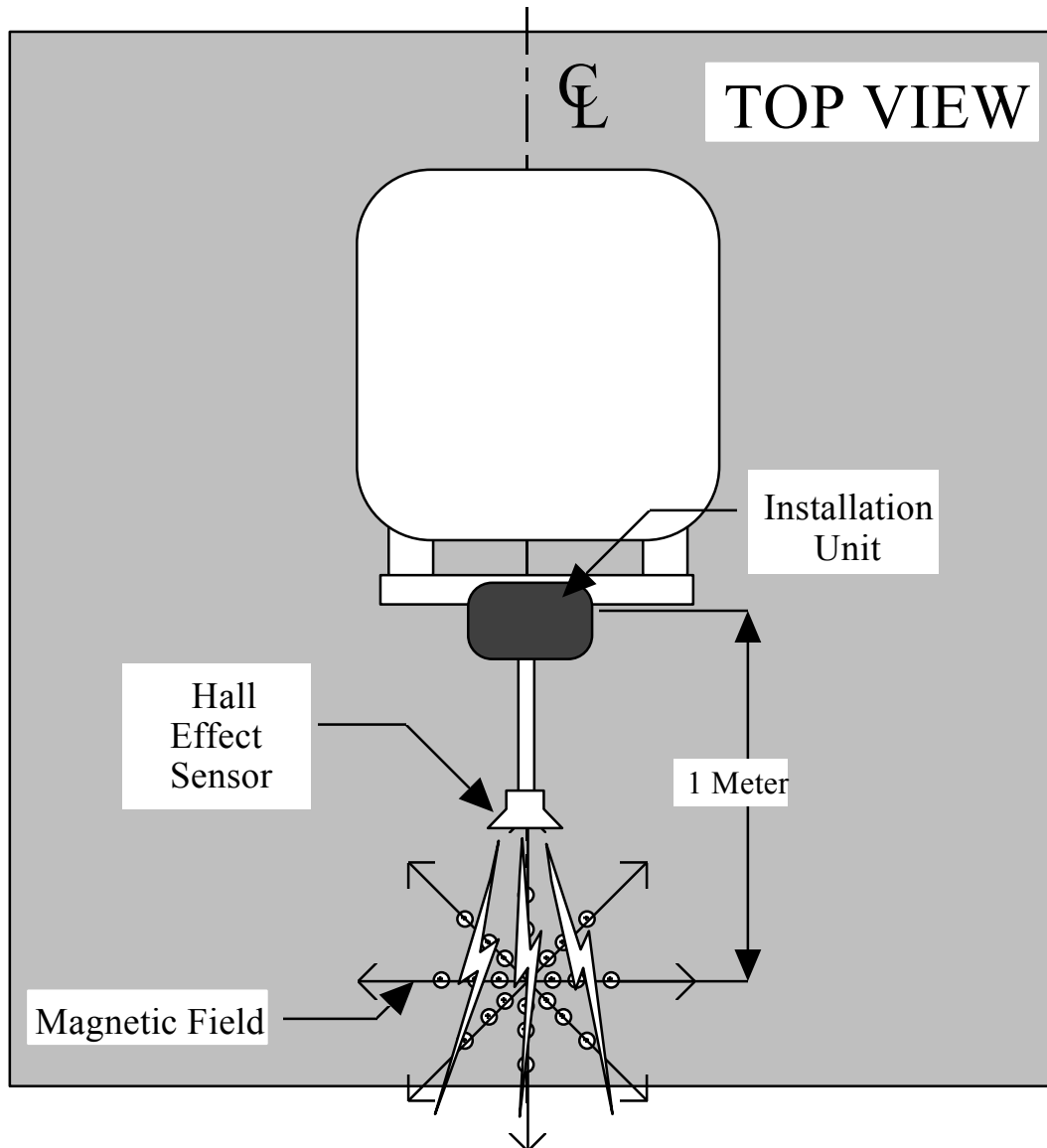
Figure 21. Hall-Effect system.
