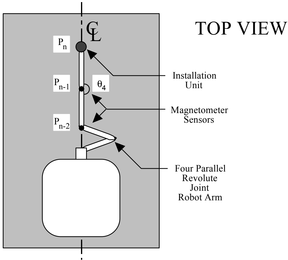
Figure 26. Installation w.r.t. the last two markers installed.
