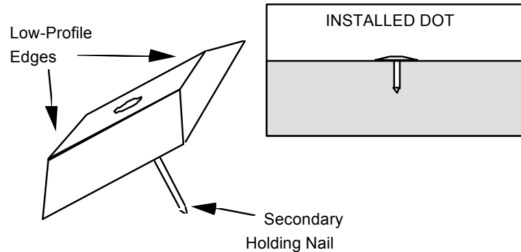
Figure 11. Magnetic dot marker.
