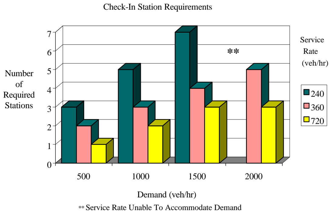
Figure 20. Check-In Station Requirements At AHS Entry
