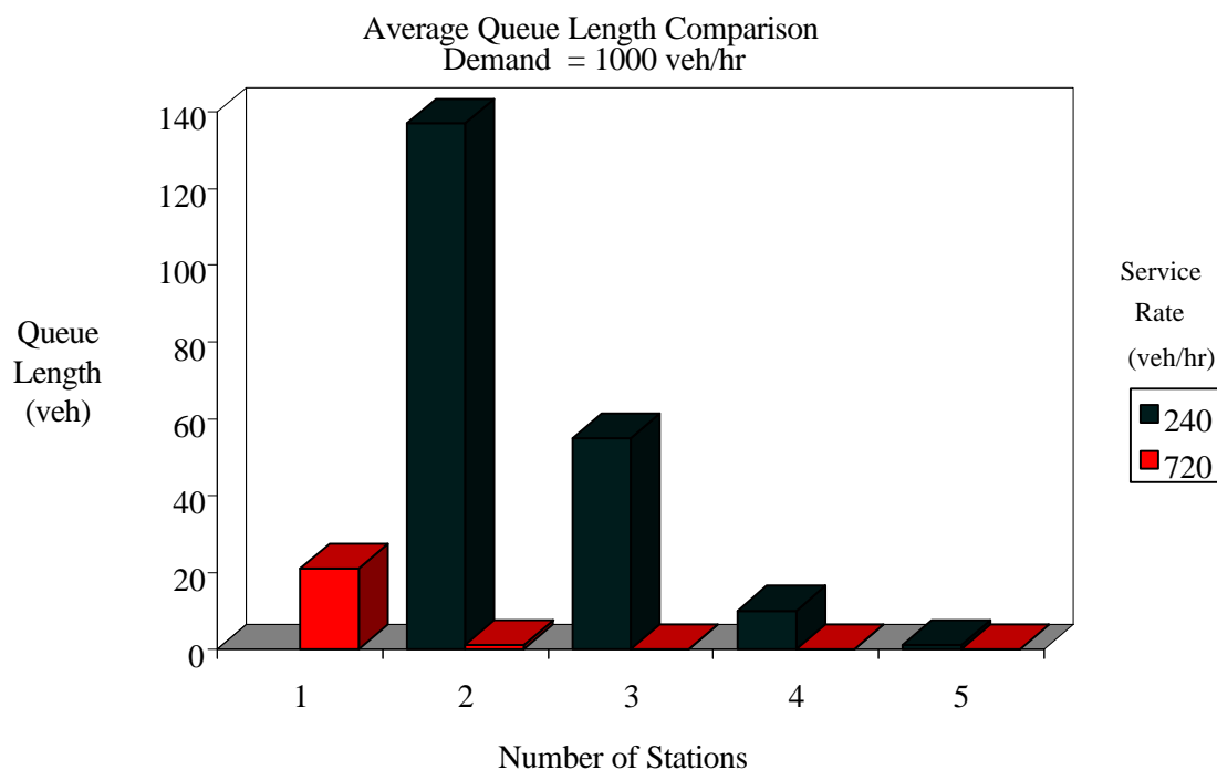
Figure 18. Average Queue Lengths For Two Service Rates
