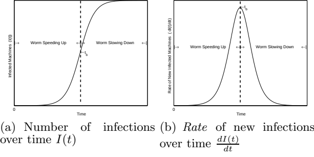
Figure 2: (a) shows infections as a function of time. (b) shows the rate of new infections. As shown, t_b divides the lifetime of a worm into two phases: acceleration and deceleration.
