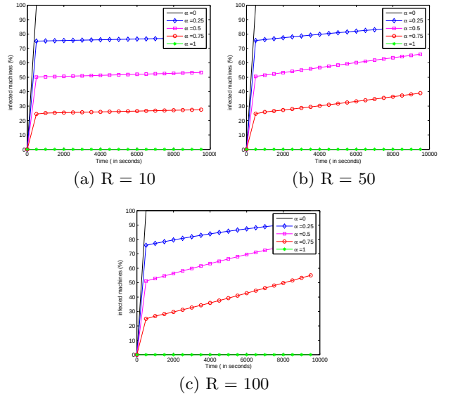
Figure 7: Effect of the sensitivity threshold on hardened Proactive Protection
