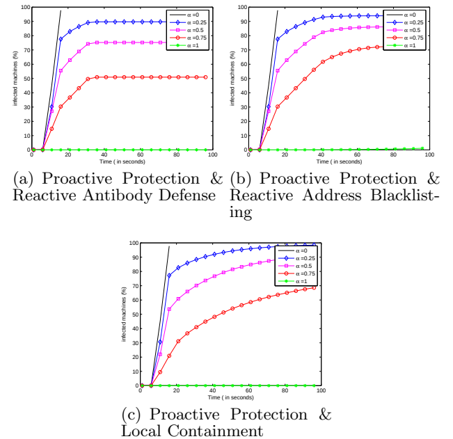
Figure 9: Hybrid defense against a Slammer worm using hit-list scanning with \delta_a = \delta_b = 30 seconds.
