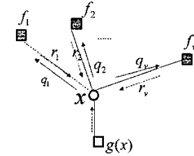
Fig. 4. Message updating around variable node
