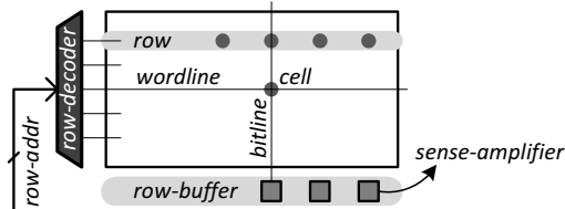
Figure 3. DRAM Bank: Logical organization
