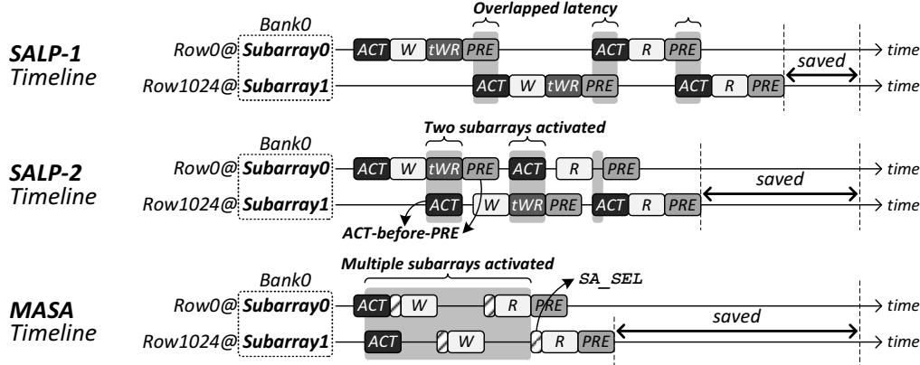
Figure 8. Service timeline of four requests to two different rows. The rows are in the same bank, but in different subarrays.
