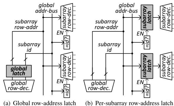
Figure 10. SALP-2: Latched Subarray Row-Decoding
