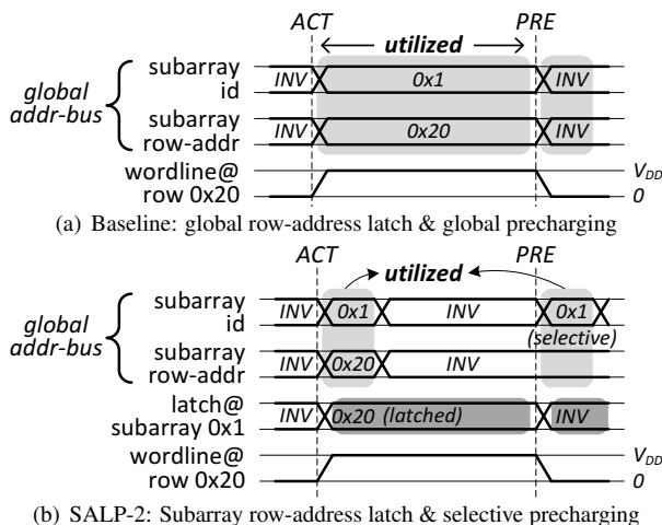
Figure 11. Activating/precharging wordline-0x20 of subarray-0x1.
