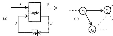
Fig. 1: The FSM model
