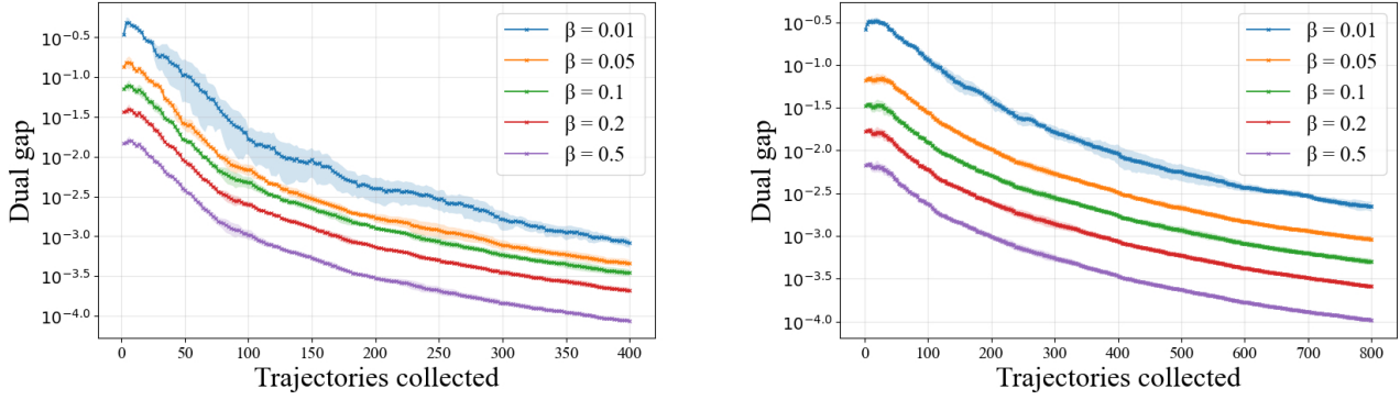
(a) H = 4, |S| = 7, A_1 = A_2 = 7, d = 5
