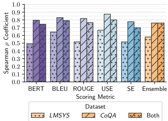
Figure 6: At response to response-set level, existing metrics and our ensemble method correlates better with human ratings on CoQA than LMSYS .
