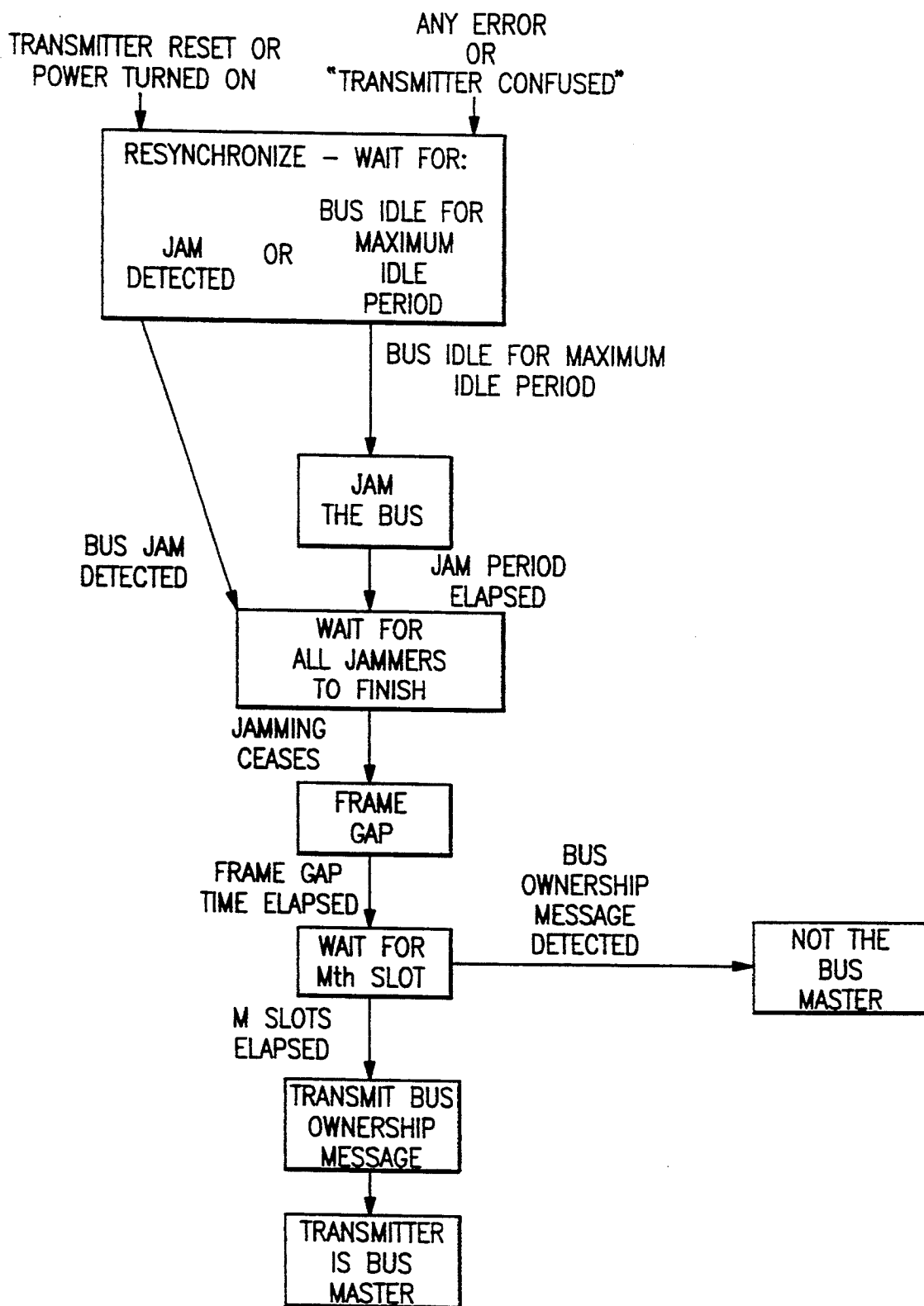
FSD FOR BUS MASTER ARBITRATION.
