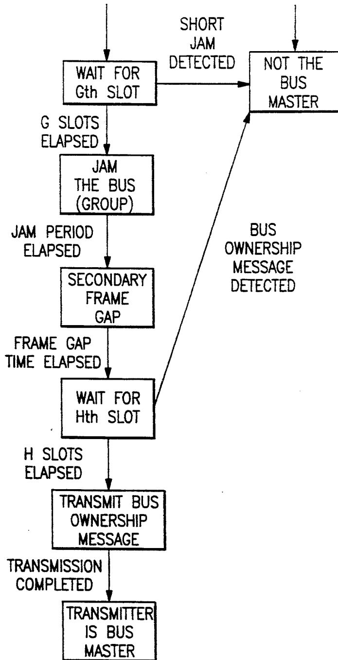
FSD FOR MULTI-LEVEL BUS MASTER ARBITRATION.
