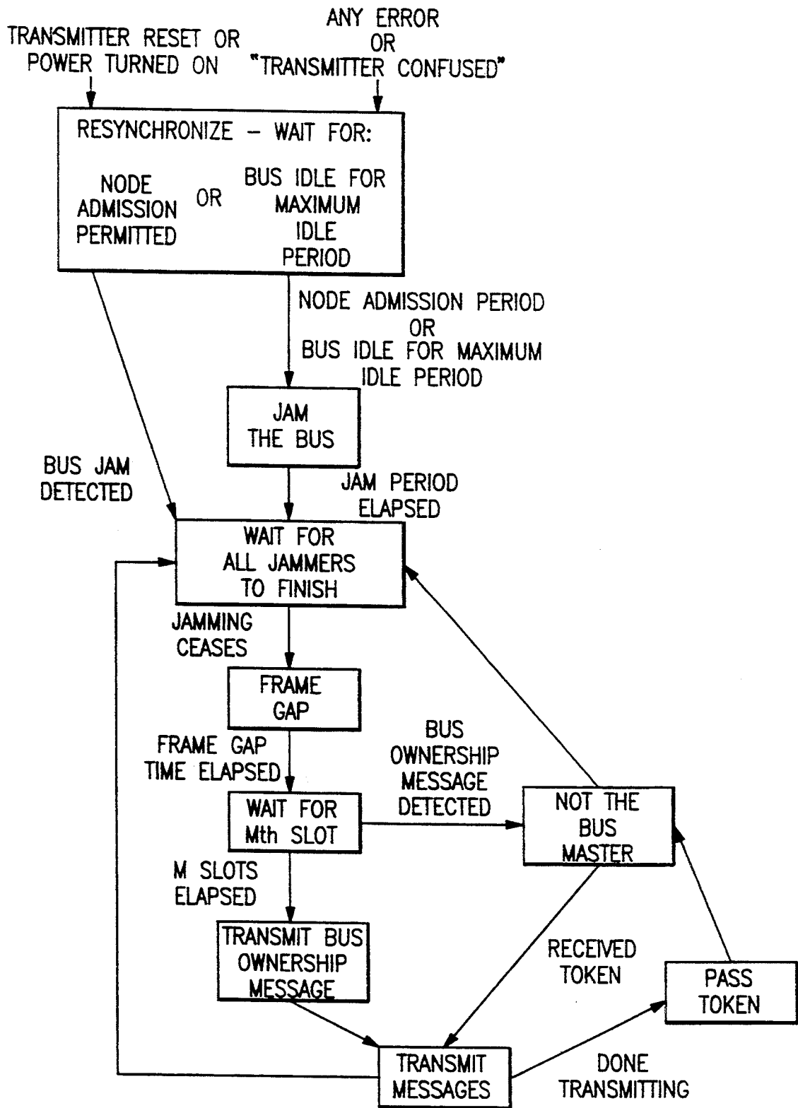
FSD FOR EXPLICIT TOKEN BUS PROTOCOL.
