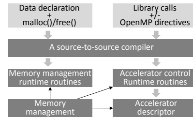
Figure 6: The overview of underlying software support to enable MEALIB portability.
