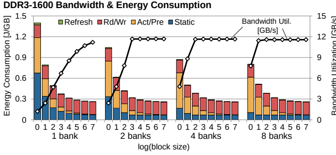
Fig. 4. Locality/parallelism vs. bandwidth, power and energy tradeoffs for DDR3-1600 DRAM (1.5V, single rank, 8 bank, x8 width) [12].
