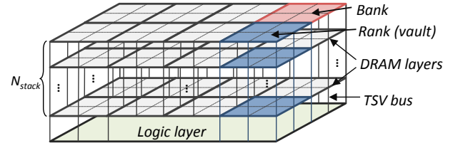
Fig. 5. Overview of the 3D-stacked DRAM organization.
