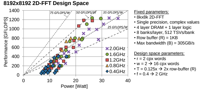
Fig. 9. Design space exploration for 2D-FFT with 3D-stacked DRAM. Isolines represent the constant power efficiency in Gflops/W (see labels).
