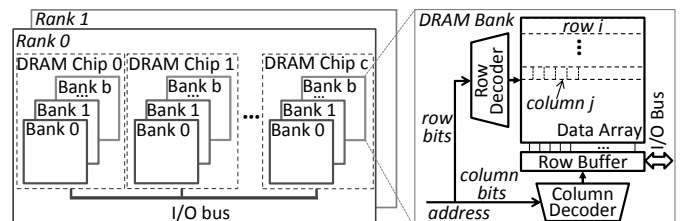
Fig. 3. Overview of off-chip DRAM organization.
