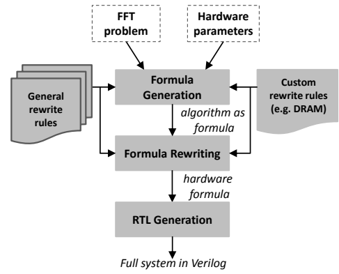
Fig. 7. Overview of the design generator tool.
