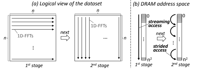
Fig. 1. Overview of row-column 2D-FFT computation.
