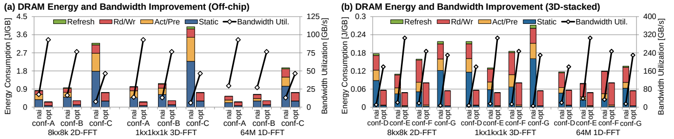
Fig. 13. DRAM energy and bandwidth utilization for naive (nai) and DRAM-optimized (opt) implementations of selected FFTs and memory configurations.
