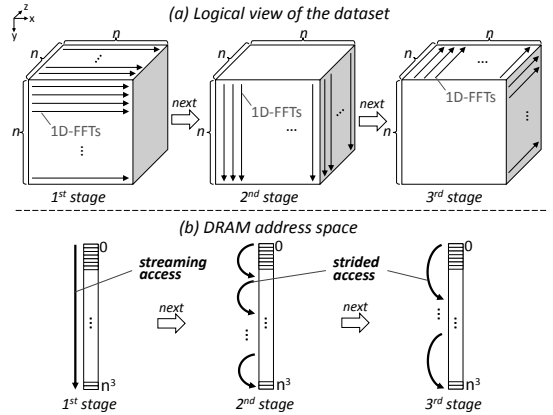
Fig. 2. Overview of 3D-decomposed 3D-FFT computation.
