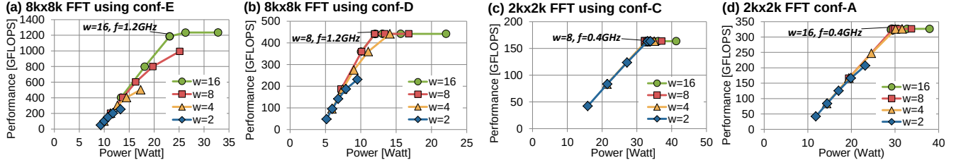
Fig. 11. Frequency ( f ) and streaming width ( w ) effects on power and performance for various problem/platform configurations (fixed tile size). Parameter combinations for the best design (GFLOPS/W) are labelled.
