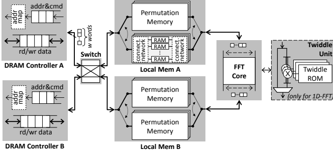
Fig. 8. Overall view of the targeted architecture.
