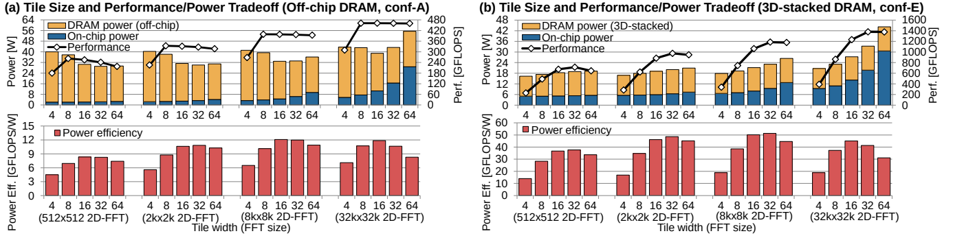
Fig. 10. Effect of tile size on performance and power efficiency for off-chip and 3D-stacked DRAM systems. (Rest of the parameters are fixed.)
