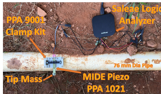
Figure 2. MIDE PPA 1021 piezo attached on 76 mm diameter pipe along with logic analyzer
