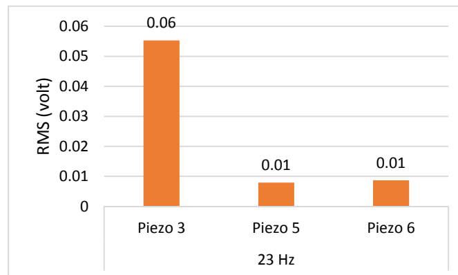
Figure 6. Comparison of RMS at straight section, before and after smooth bend
