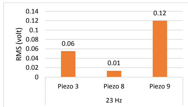
Figure 7. Comparisons of RMS at straight section, before and after 90° bend
