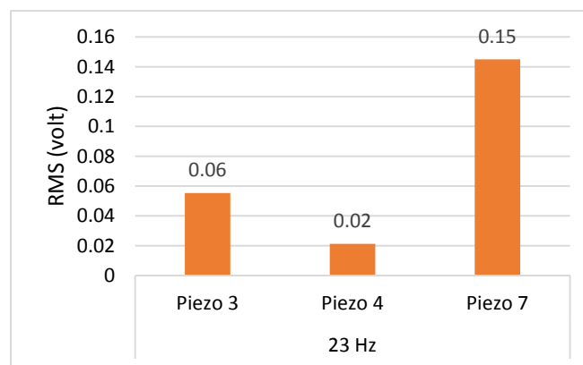
Figure 8. Comparisons of RMS at straight section, before and after Tee bend
