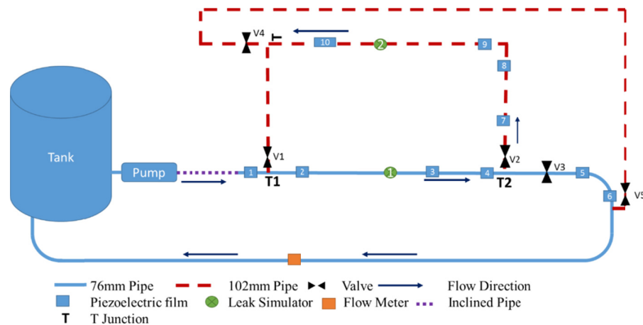
Figure 1. Schematic layout of the experimental pipeline set-up
