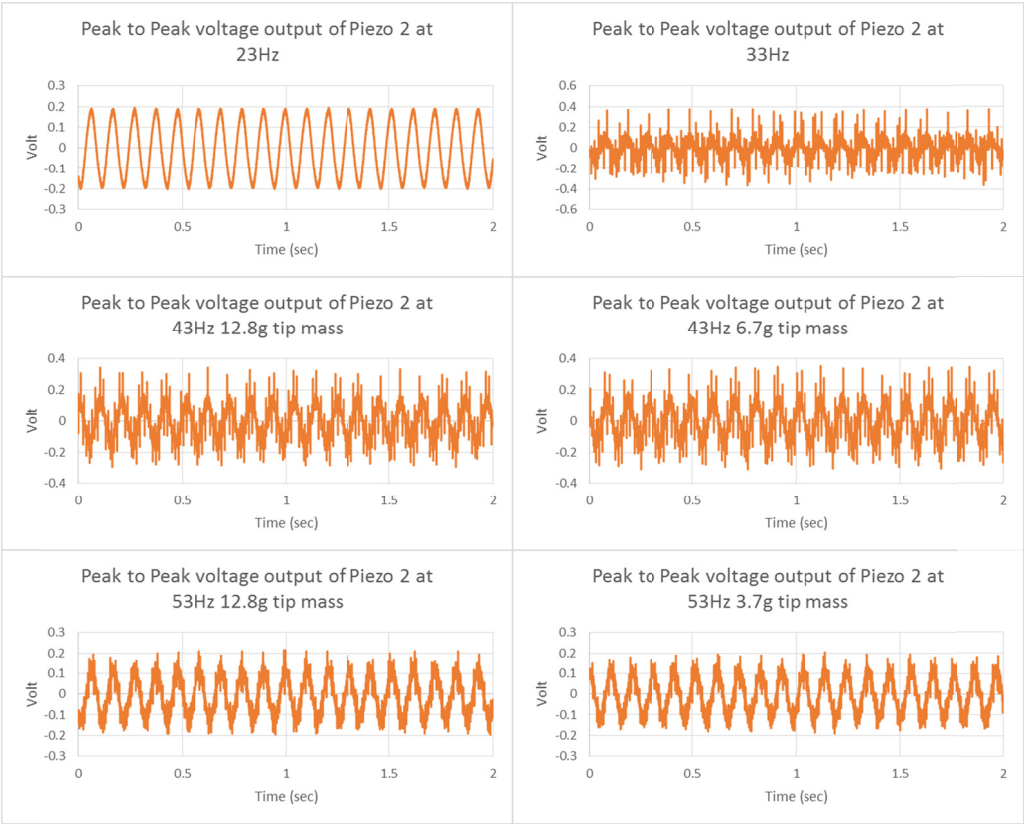
Figure 4: Peak to peak voltage output of piezo #2 at 23Hz, 33Hz, 43Hz, and 53Hz pump frequencies and different tip masses
