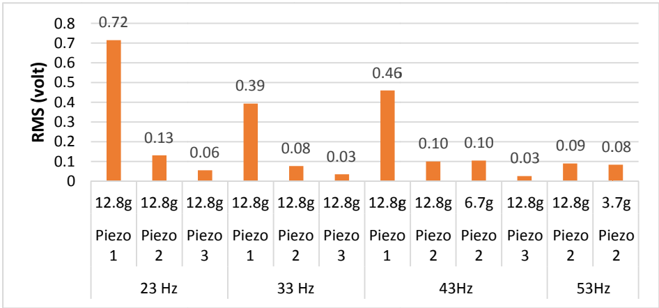
Figure 3. Comparison of RMS (volt) at different locations on straight section
