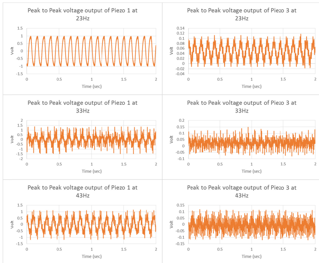
Figure 5: Peak to peak voltage output of piezo #1 and piezo #3 at 23Hz, 33Hz, and 43Hz with 12.8-gram tip mass
