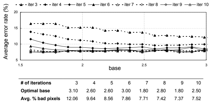
Fig. 8. Error rate of ESMP for varying b and iteration numbers.
