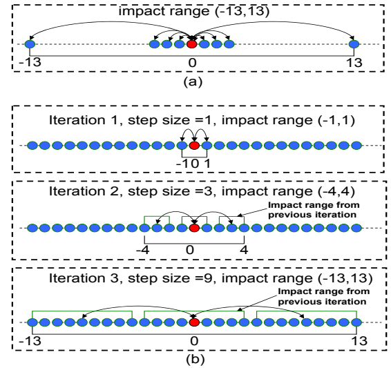
Fig. 2. A 1-D example of cost aggregation: (a) conventional aggregation used in [5], (b) exponential step size information propagation.
