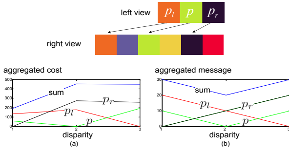
Fig. 6. A synthesized example showing difference of aggregating matching costs and aggregating messages. Ground truth disparity of pixel p is 2. (a) blue curve shows the result of aggregating matching costs for p , where minimum is reached at disparity 1. (b) blue curve shows the result of aggregating messages for p , where minimum is reached at true disparity 2. Messages are computed from matching costs using equation (11). In this example, V(x) = 10|x| .
