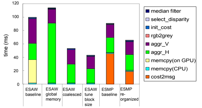
Fig. 12. Profile of execution time of different implementations on Teddy dataset, at iteration 9. (Best view in color)
