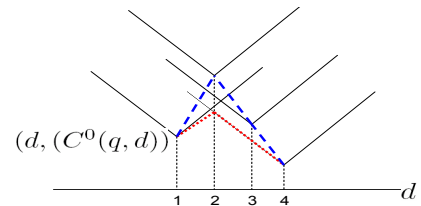
Fig. 5. An illustration of min-sum computation (without truncation). Output M(q, d) is the lower envelop of four Cones rooted at (d, C^0(q, d)) . Dashed blue curve shows C^0(q, d) , dotted red curve shows the lower envelop.
