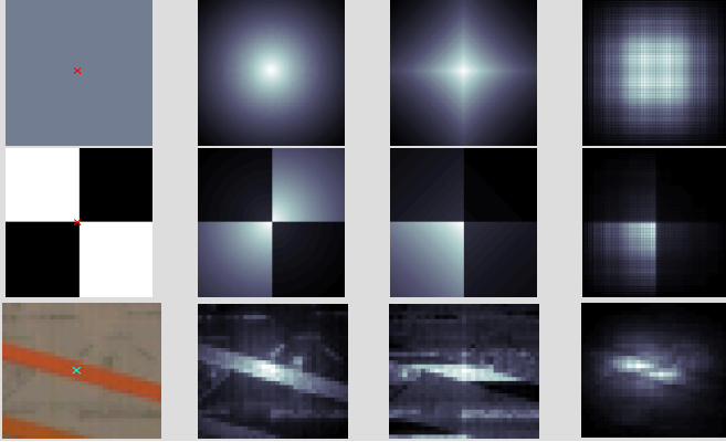
Fig. 1. From left to right: sample window, AW[23], RtAW[5] and ESAW.
