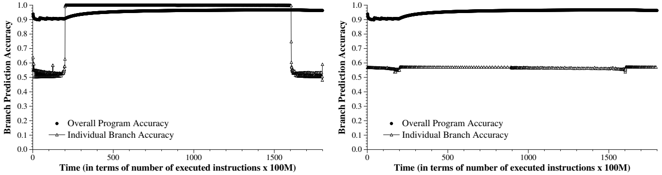
Figure 8. The time-varying phase behavior of the prediction accuracy of an input-dependent branch (left) vs. an input-independent branch (right) from the gap benchmark
