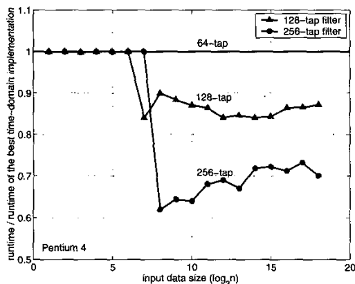
Fig. 3. Runtime improvement using frequency-domain algorithms.
