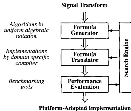
Fig. 1. The architecture of SPIRAL.
