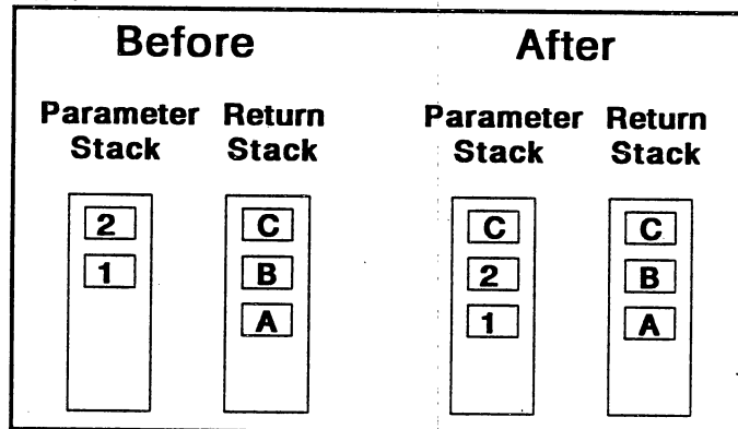
FIGURE 3.10: STACK EFFECTS OF R@
