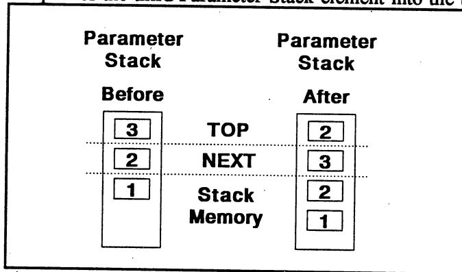
FIGURE 3.7: STACK EFFECTS OF OVER
