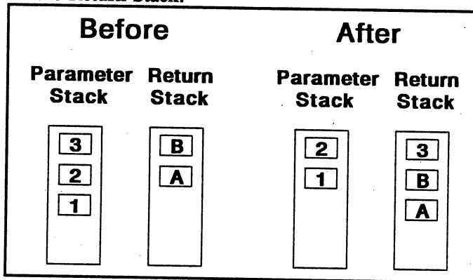
FIGURE 3.8: STACK EFFECTS OF >R
