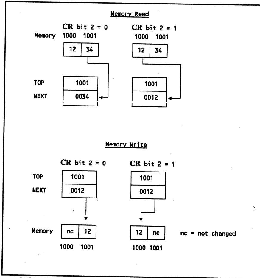
FIGURE 5.9: 8-BIT READ/WRITE TO ODD MEMORY ADDRESS
