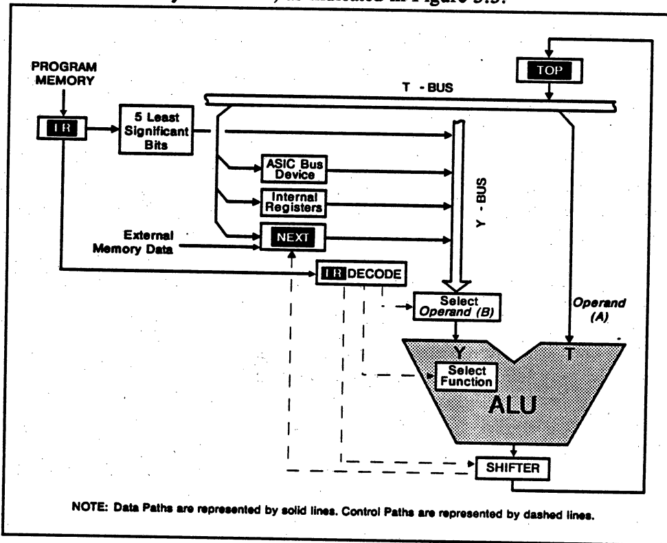
FIGURE 3.3: ALU DATA FLOW
