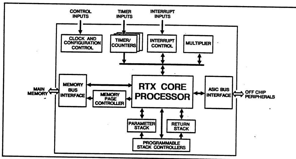
FIGURE 2.1: RTX 2000 BLOCK DIAGRAM
