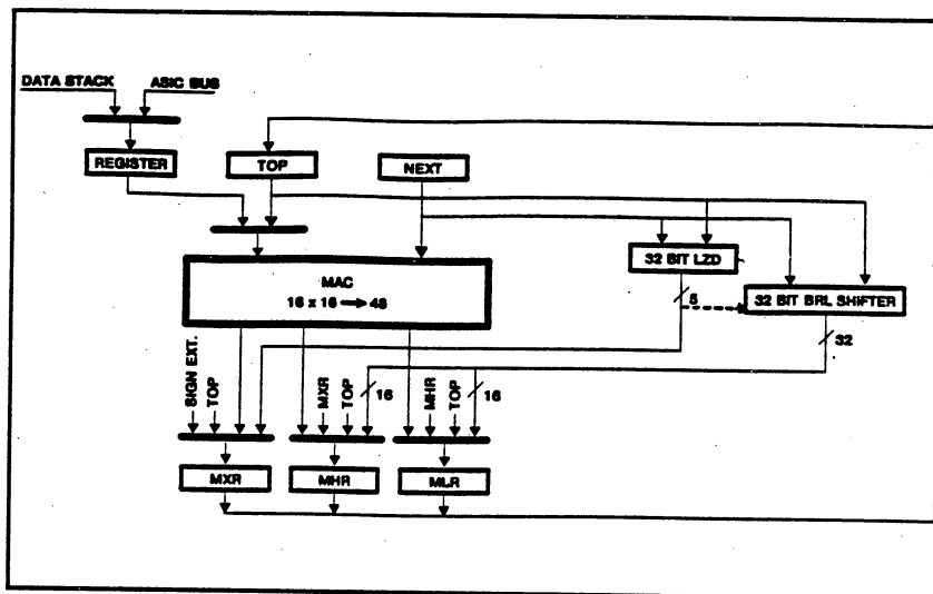
FIGURE 6.9: RTX 2010 FLOATING POINT/DSP LOGIC
