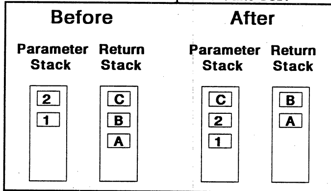
FIGURE 3.9: STACK EFFECTS OF R>
