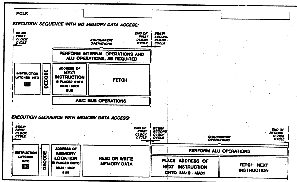
FIGURE 3.1: INSTRUCTION EXECUTION
