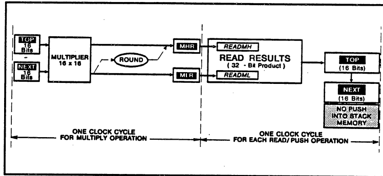
FIGURE 6.8: RTX 2000 MULTIPLIER OPERATION
