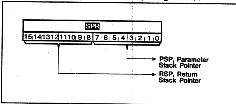
FIGURE 6.2: RTX 2000 STACK POINTER REGISTER
