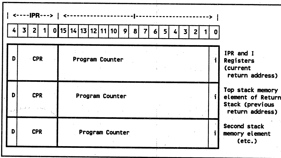
FIGURE 5.2: RETURN STACK STRUCTURE
