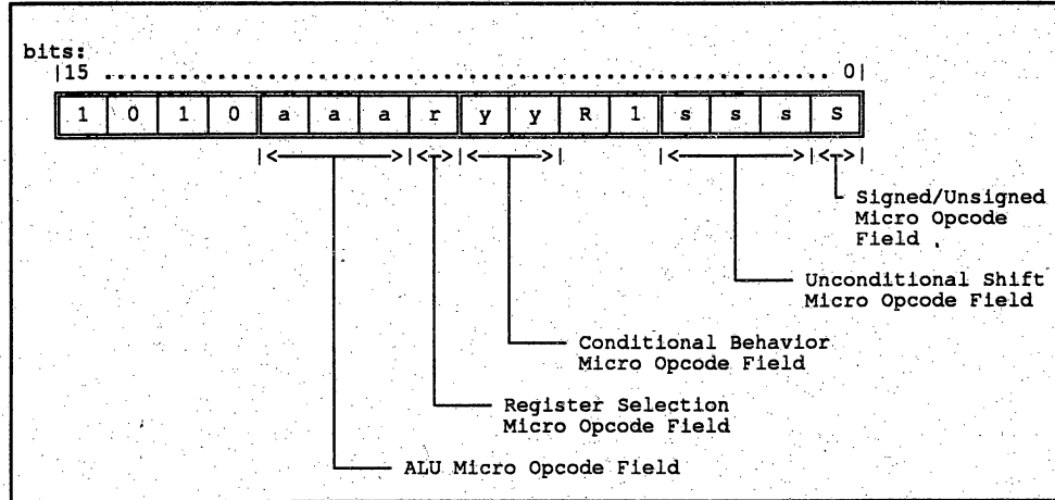
FIGURE 8.2: STEP MATH INSTRUCTION FORMAT
