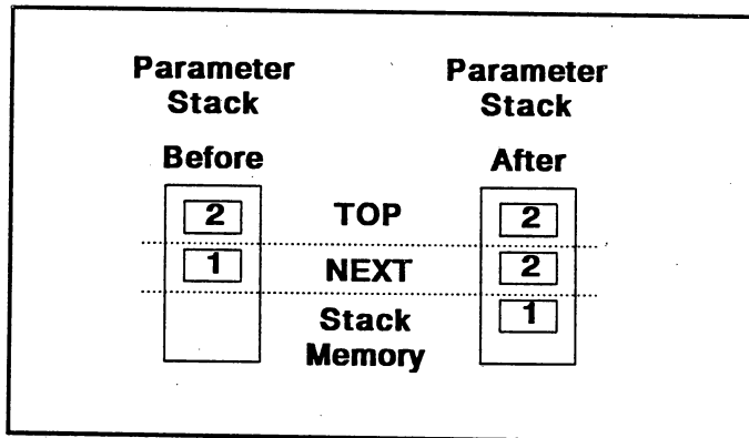
FIGURE 3.4: STACK EFFECTS OF DUP
