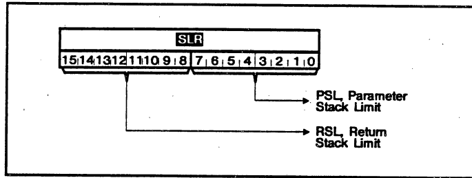
FIGURE 6.6: RTX 2000 STACK LIMIT REGISTER
