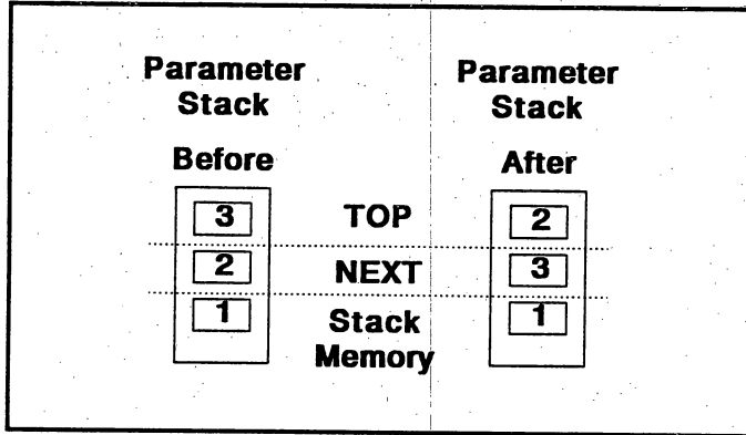
FIGURE 3.5: STACK EFFECTS OF SWAP
