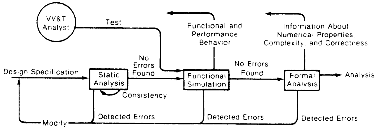
Figure 3.3 Integrated approach to design VV&T
