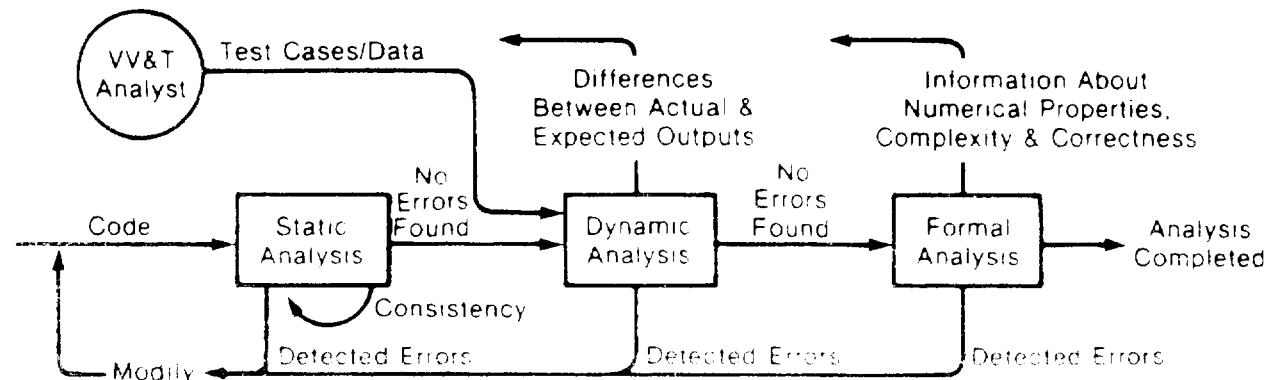
Figure 3.4 Integrated approach to code VV&T
